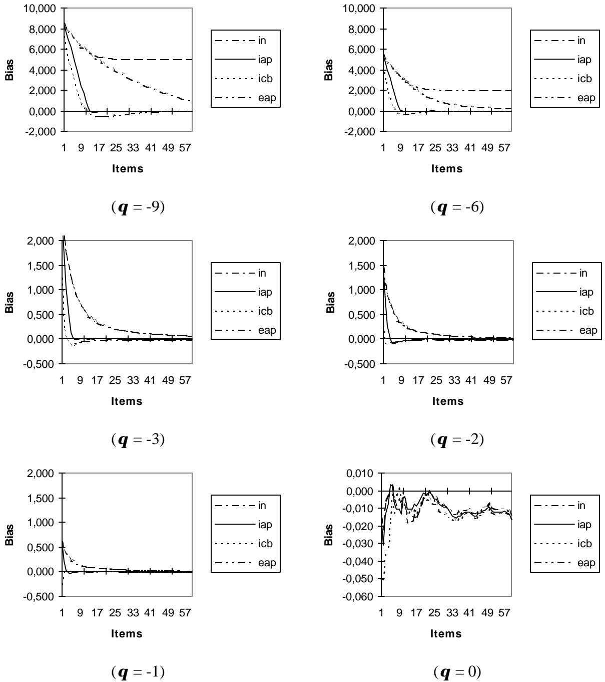
Figure 1. Bias of the proficiency estimate according to the number of items administered
